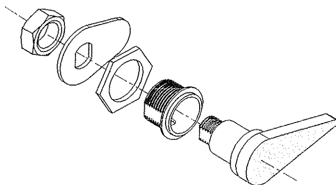
DL-95 Tear Drop Latch Assembly
