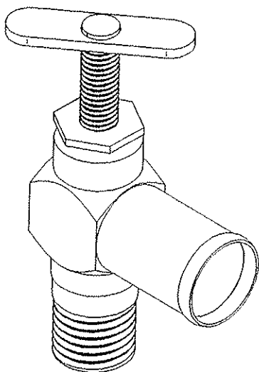
VH-054 Shut-Off Valve 5/8" Hose x 3/8" Male Pipe Qty: 1
