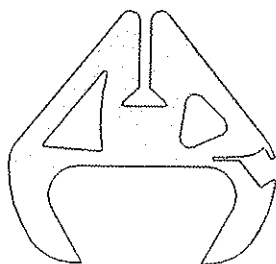
WE-620-0013 Glazing Rubber for Thermopane Glass
