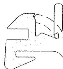
ST-1205R046 Self Locking Glazing Rubber
