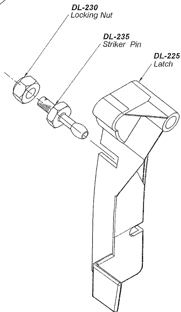
Latch Assembly
